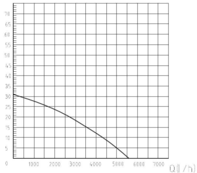
H(m) LIFT 30
