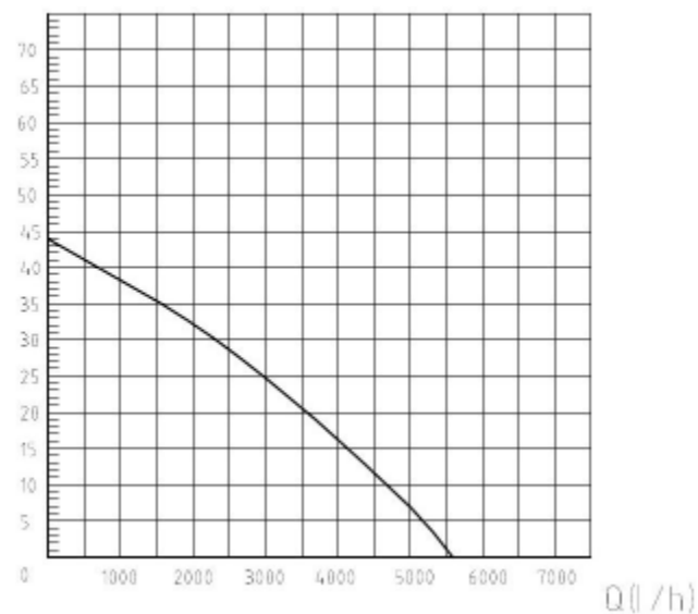
H(m) LIFT 40
